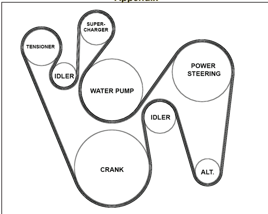
2010-2012 Belt Routing Diagram
